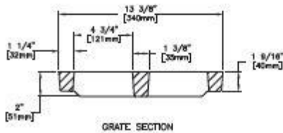
GRATE SECTION
