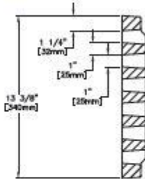
GRATE SECTION
